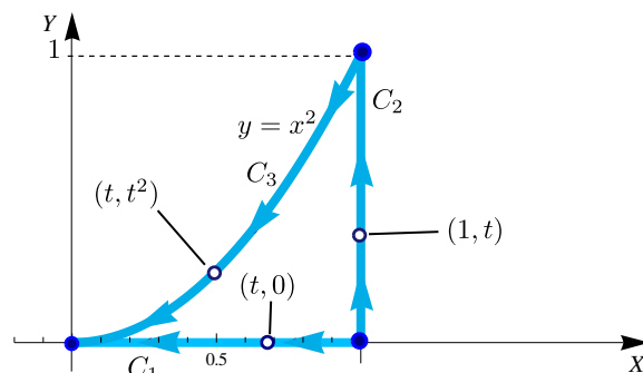
Figura 9.16: Curva C = C_1 \cup C_2 \cup C_3 .
