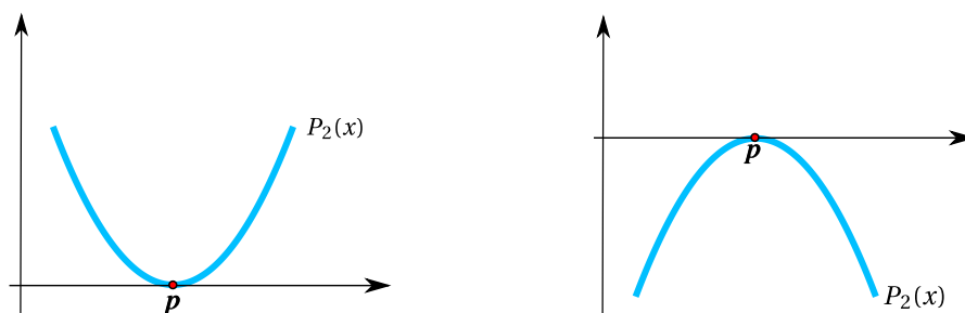
Figura 6.2: Parábolas f''(\mathbf{p})(\mathbf{x} - \mathbf{p})^2 con f''(\mathbf{p}) > 0 y f''(\mathbf{p}) < 0
