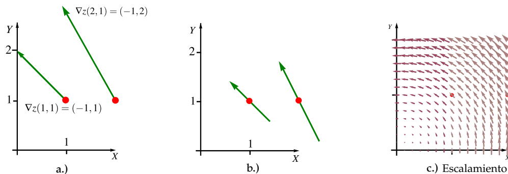
Figura 8.6: Campo F(x, y) = (-y, x)
