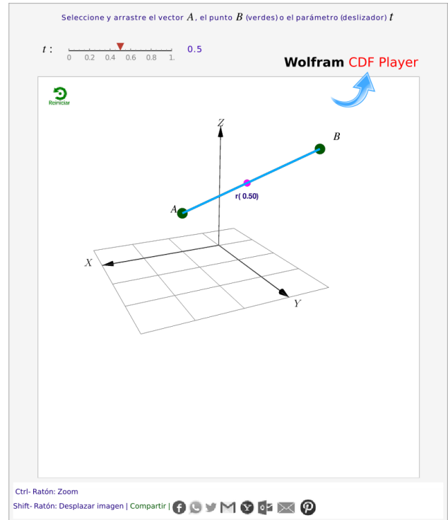
Figura 4.8: C: \mathbf{r}(t) = A + t \cdot (B - A), t \in [0, 1]
