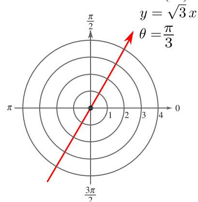
Figura 1.35: Recta \theta = \frac{\pi}{3}
