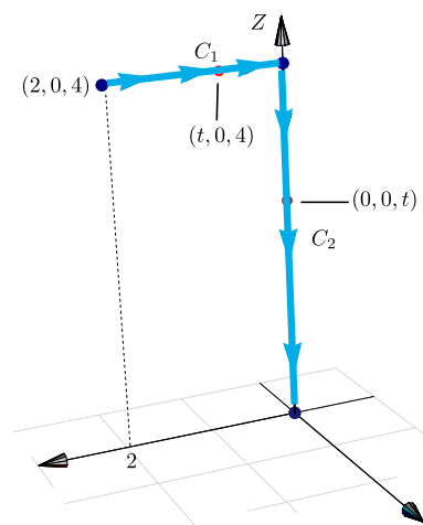
Figura 9.22: Curva C' = C_1 \cup C_2 .
