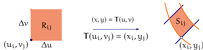
Figura 7.31: f(x_i, y_i) A_{S_{ij}} \neq f(\mathbf{T}(u_i, v_j)) \Delta u \Delta v
