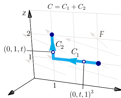
Figura 9.17: Curva C = C_1 \cup C_2 .
