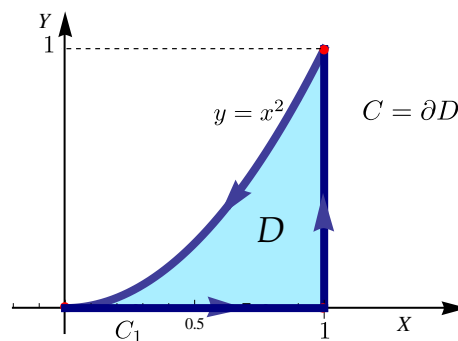
Figura 9.24: Curva C = C_1 \cup C_2 \cup C_3 .
