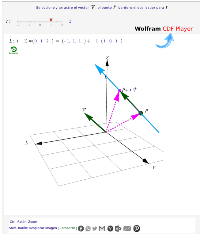
Figura 4.7: L: \mathbf{r}(t) = P + t\vec{v}, t \in \mathbb{R}
