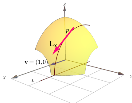
Figura 5.22: \mathbf{v} = (1, 0)
