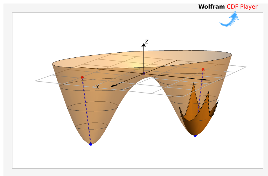
Figura 6.10: f(x, y) = x^4 + y^4 - 2x^2 + 4xy - 2y^2
